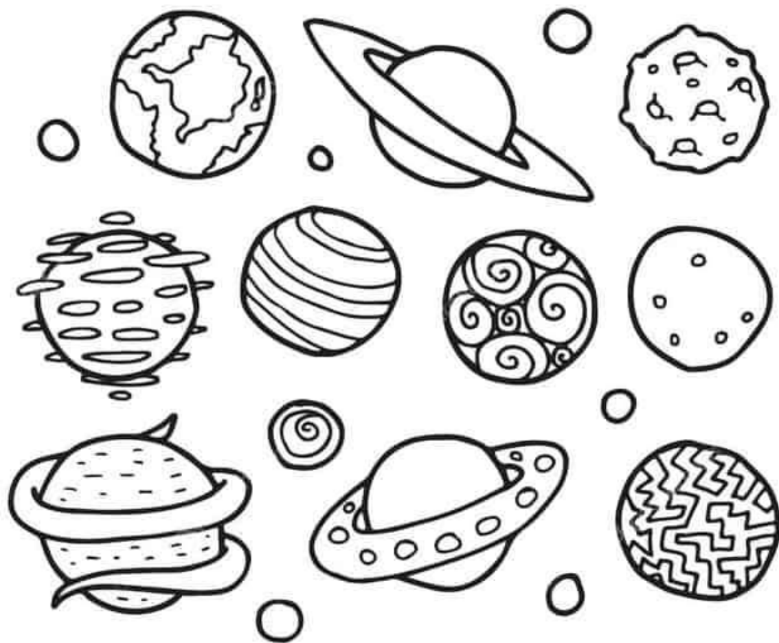
planet set
