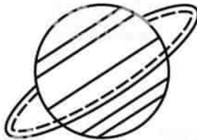
SATURN
